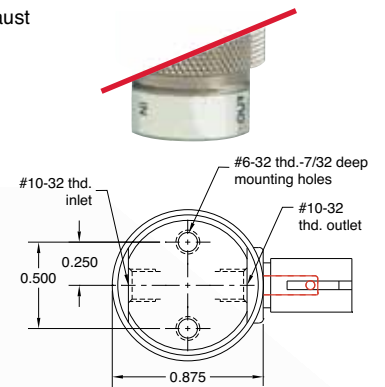
3-Way Fully-Ported In-Line Mount
