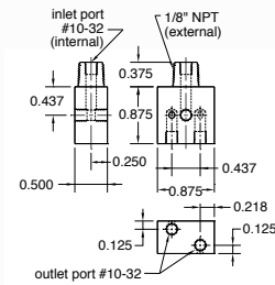
Part No. 15490-3 Description 1/8" NPT Inlet, #10-32 Outlet
