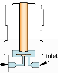
2-Way Normally-Closed High Flow
