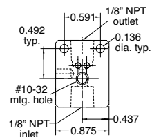
Part No. 15490-5 Description 1/8" NPT Inlet, 1/8" NPT Outlet
