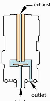
3-Way Normally-Closed Manifold Mount
